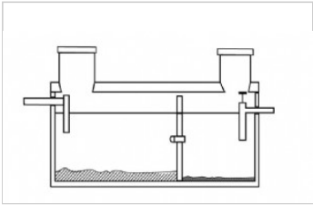
Septic tank two compartment center baffle configuration
