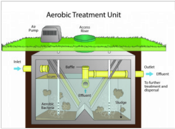
Aerobic treatment unit ATU system: aeration, clarification, profile view, color
