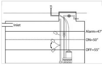
Demand dosing single differential float switch
