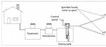
Treatment, disinfection, spray distribution
