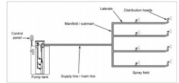
Identification of distribution system components
