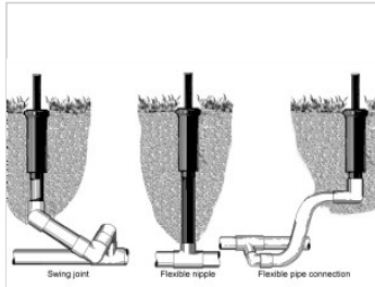
Options for connecting distribution head lateral
