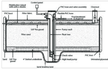
Buried single pass sand filter with pump vault Construction detail for buried, single pass sand filter with a pump vault, profile view
