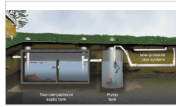
Septic tank and low pressure distribution STA
