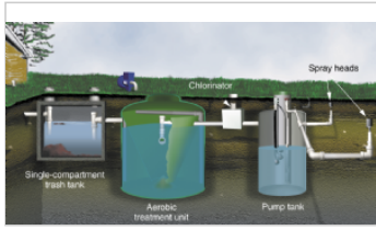
Aerobic treatment unit with surface application STA
