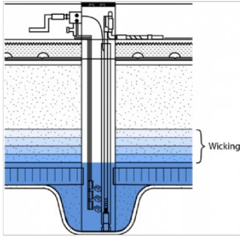
Buried single pass sand filter with pump vault
