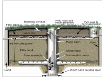
Buried sand filter unit
