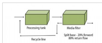
Process flow diagram Processing tank & media filter split base
