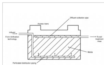
Schematic of an upflow anaerobic media filter, profile
