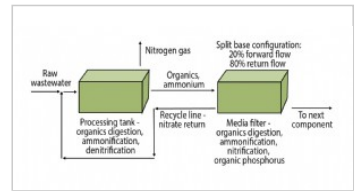
Process flow diagram Processing tank & media filter split base percent removal
