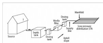
Septic tank, SP media filter, LPD distribution
