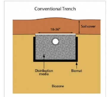
Conventional trench
