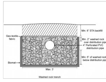
Washed rock trench cross section
