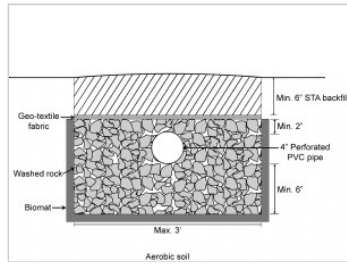
Conventional trench detail
