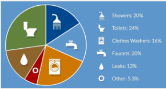
Flow contribution by fixture and usage Wastewater sources by fixture and usage
