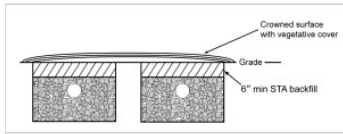
Final cover backfill over an STA
