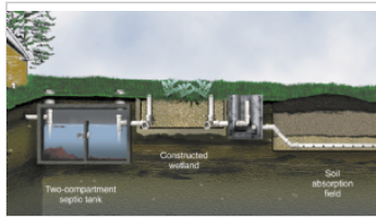
Constructed wetland system with trench distribution STA
