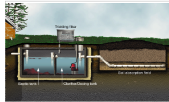
Recirculation trickling filter with trench distribution STA
