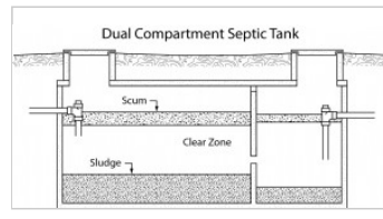
Dual compartment septic tank solids separation Two compartment septic tank showing baffle wall and solids separation, profile view
