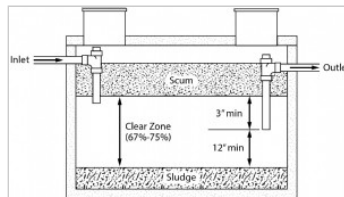
Tank pumping guidelines Guidelines for pumping septic tanks based upon sludge and scum accumulation relative to outlet baffle
