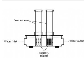
Chlorinator, tablet
