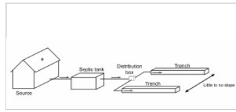
Distribution, parallel
