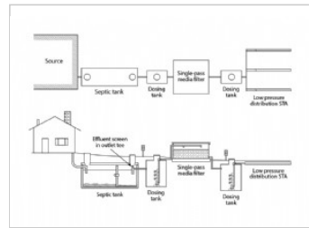
Single pass media filter to low pressure distribution STA
