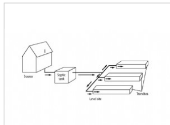
Gravity parallel trenches with manifold
