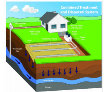
Combined treatment and dispersal system
