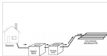
Example OWTS ST, dosing tank, LPD distribution
