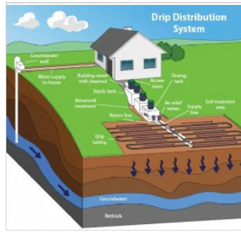
Drip distribution
