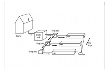
Gravity sequential trenches
