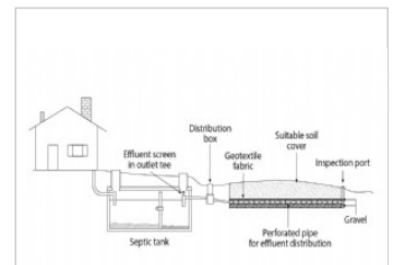
Gravity distribution system
