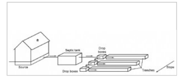
Distribution, sequential
