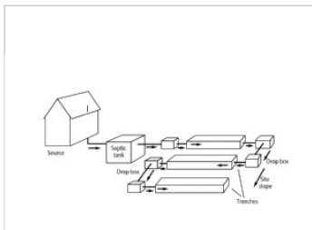
Gravity serial trenches
