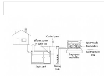
Single pass bottomless foam media filter
