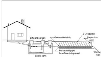
Gravity distribution system, profile
