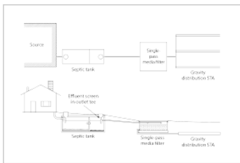
Single pass media filter gravity distribution STA
