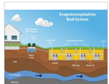
Evapotranspiration bed
