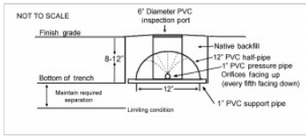
Shallow narrow trench cross section
