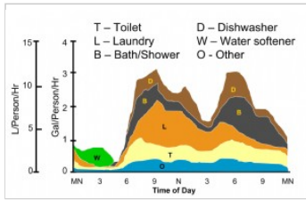
Daily fluctuation of residential wastewater source flow
