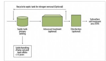
Process flow diagram to subsurface STA
