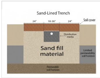
Sand lined trench perimeter description
