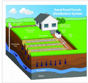
Sand lined trench gravity distribution
