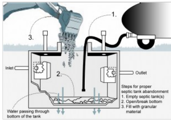
Abandonment of septic tank
