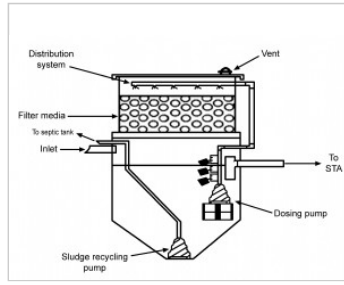
Trickling filter schematic, profile
