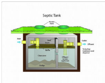
Septic Tank
