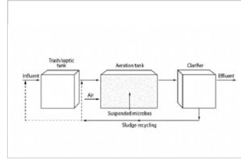
Generic suspended growth treatment process
